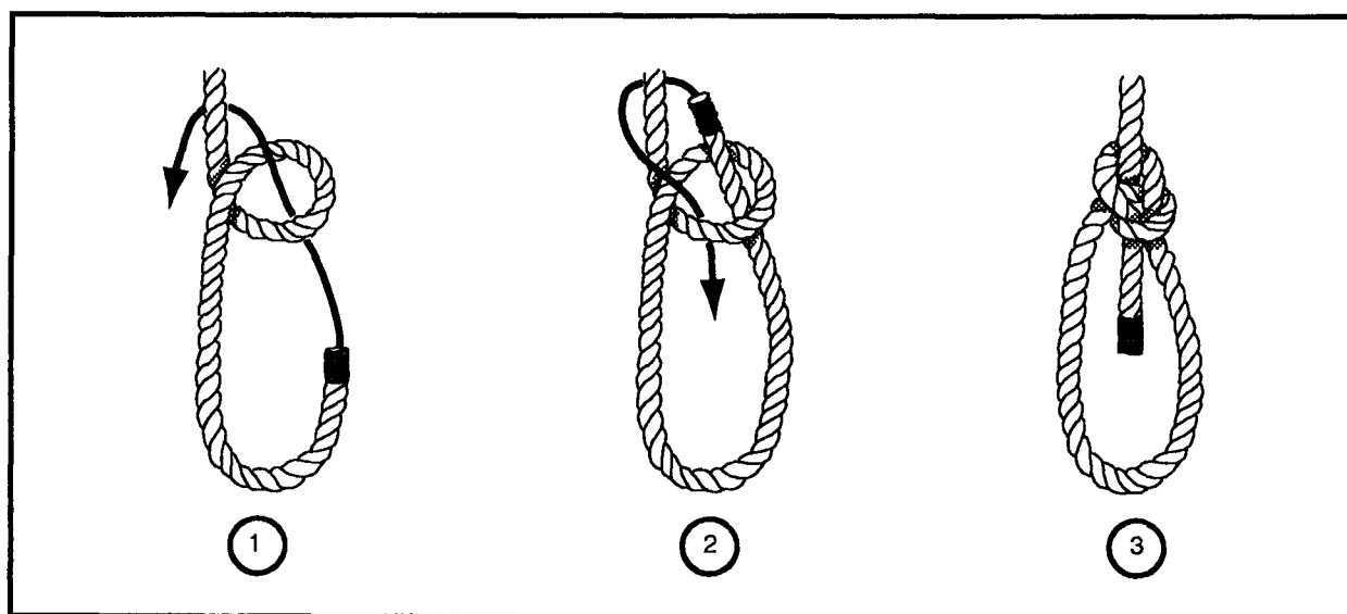
Figure 2-11. Bowline
