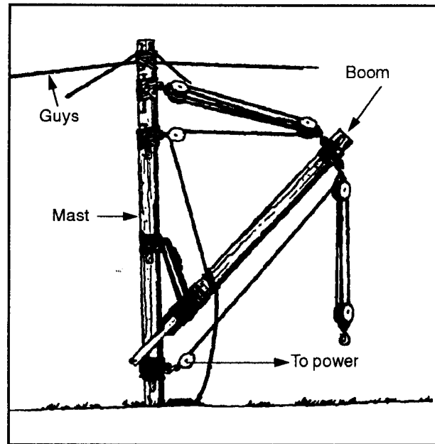
Figure 5-9. Rigging a boom on a gin pole
