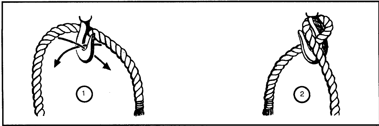
Figure 2-31. Blackwall hitch
