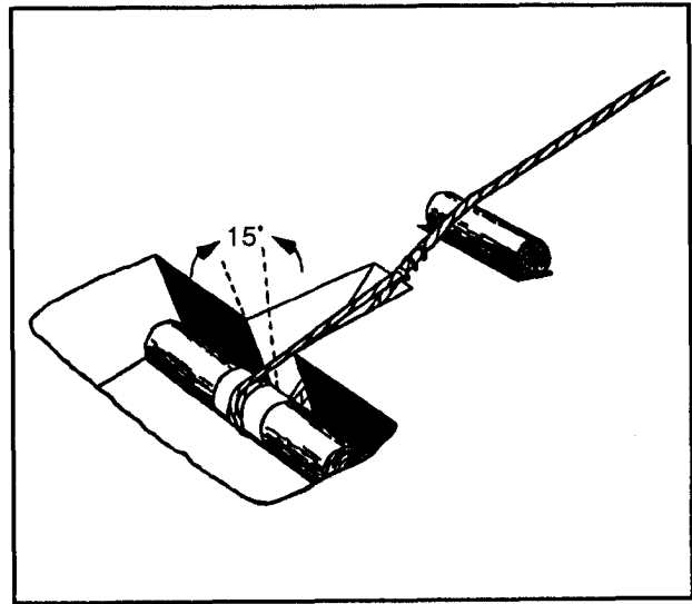
Figure 4-13. Log deadman
