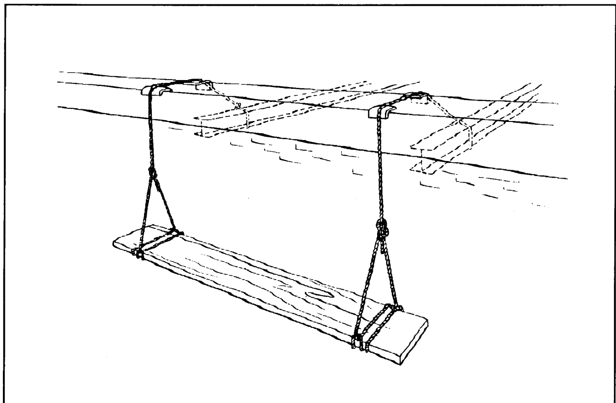
Figure 6-2. Single-plank swinging scaffold
