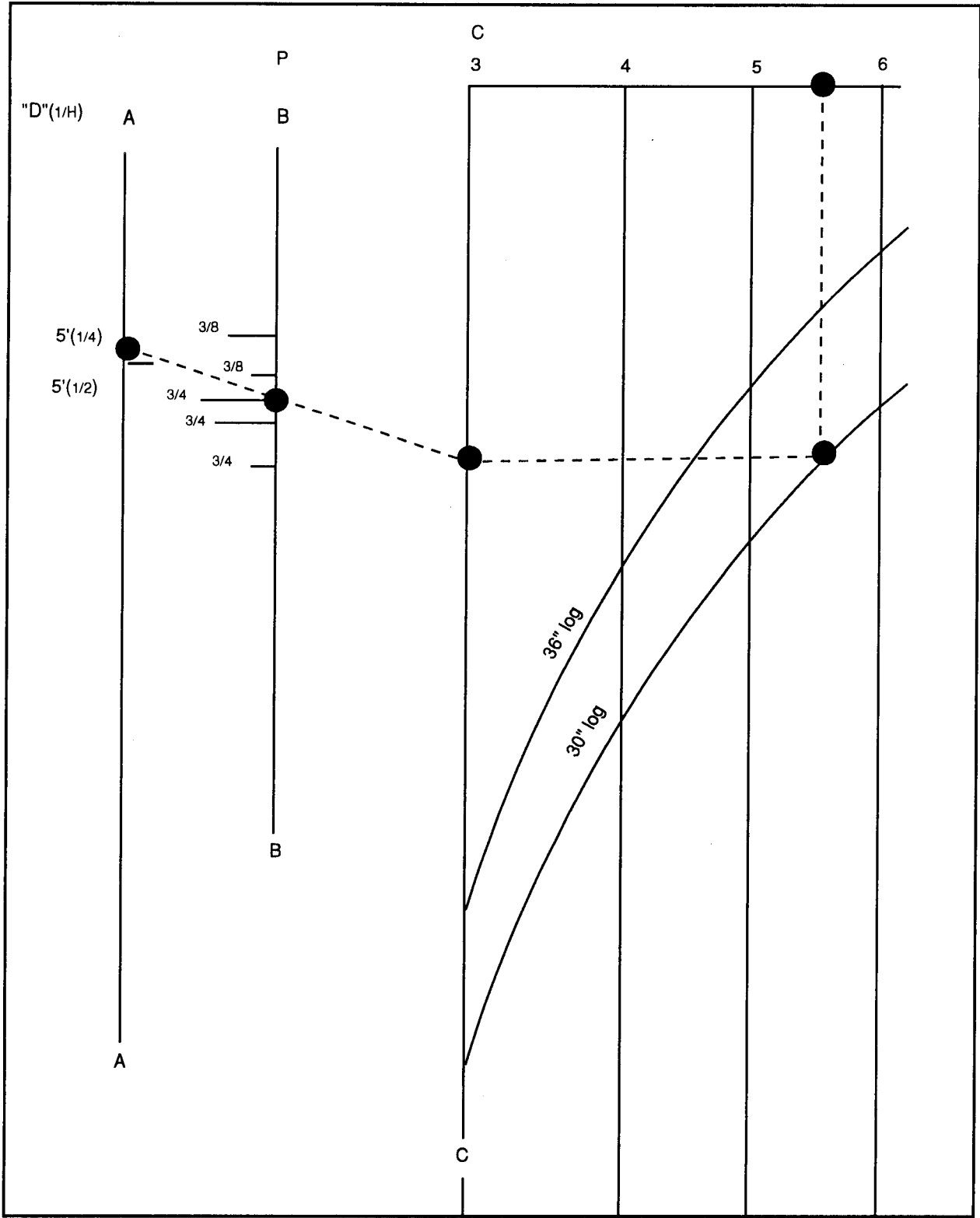
Figure 4-15. Using a nomograph
