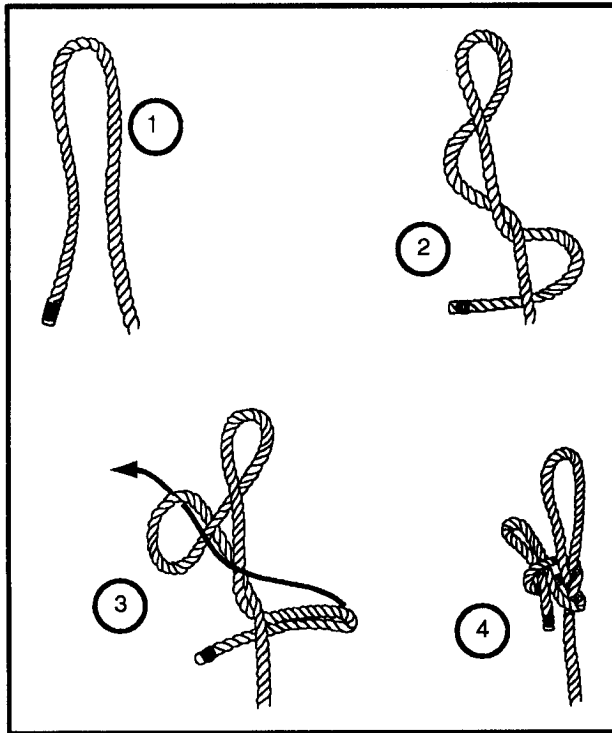
Figure 2-17. Speir knot
