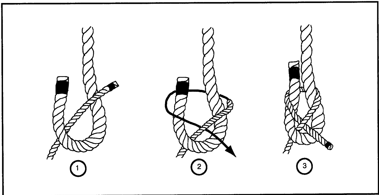
Figure 2-8. Single sheet bend
