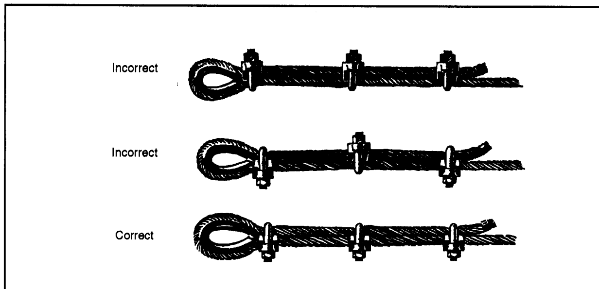
Figure 2-50. Wire-rope clips
