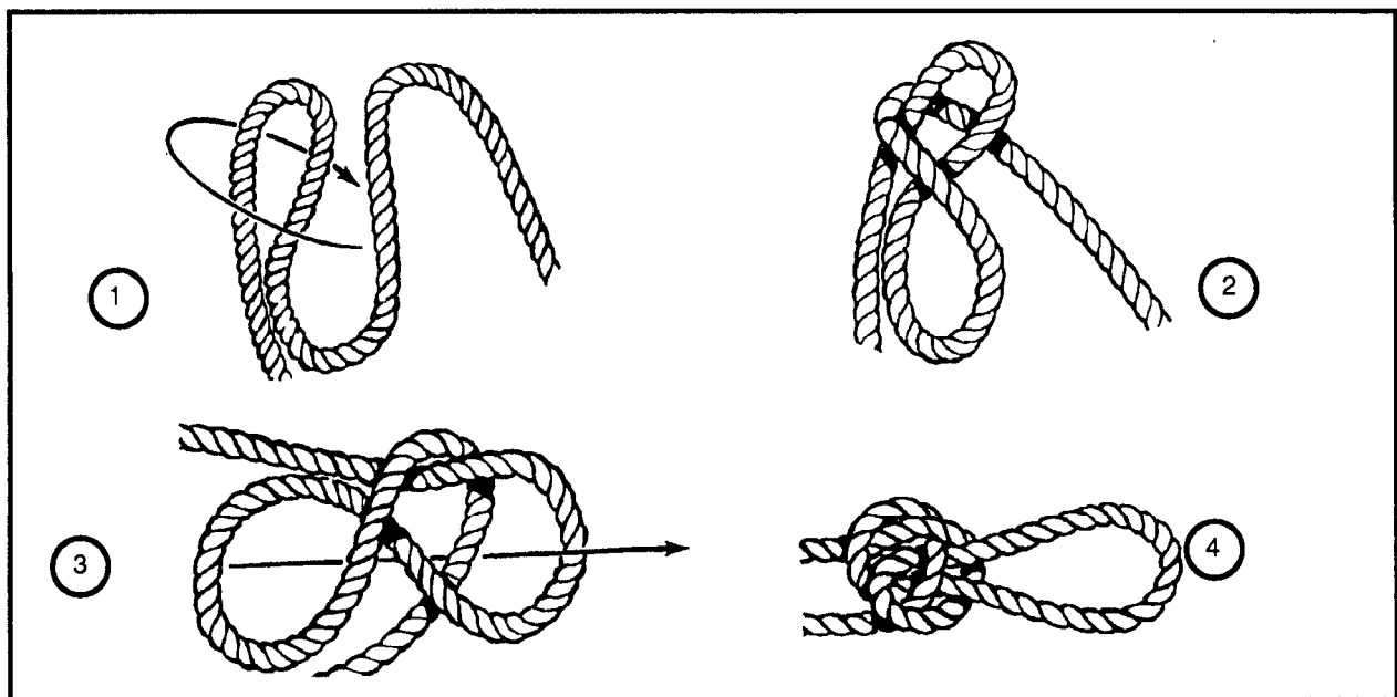
Figure 2-32. Harness hitch
