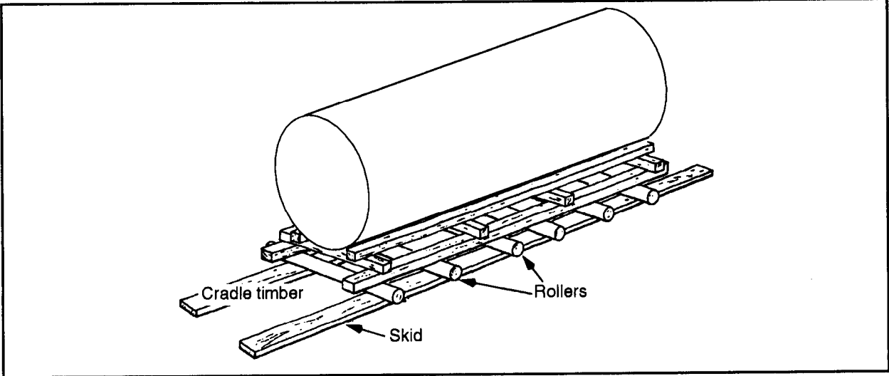
Figure 5-13. Using skids and rollers
