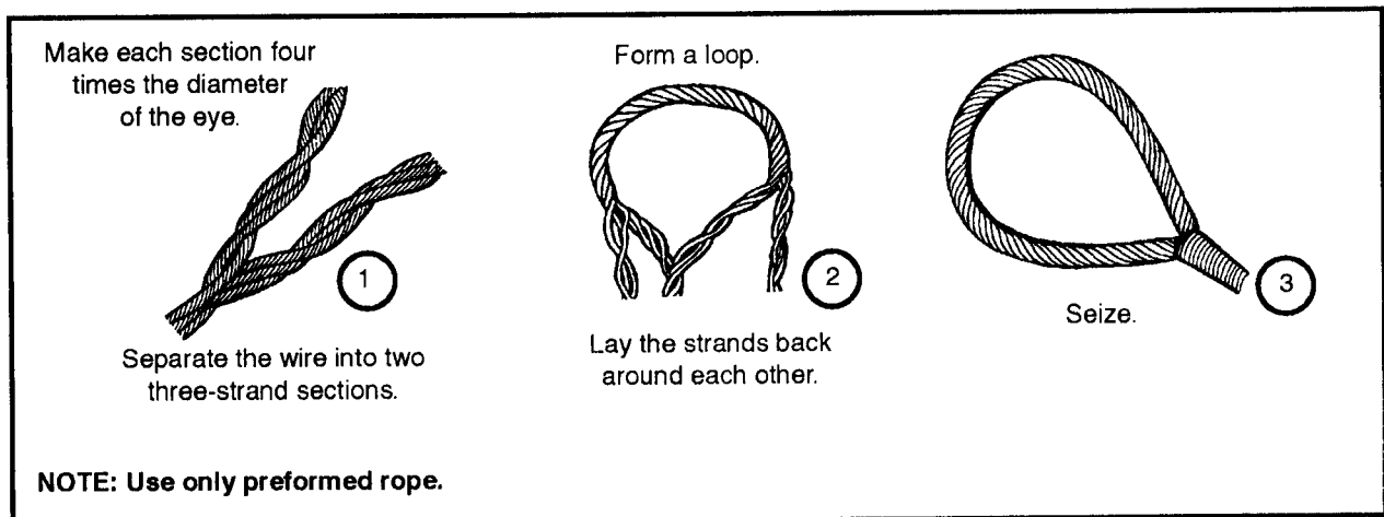
Figure 2-47. Hasty eye splice for wire rope
