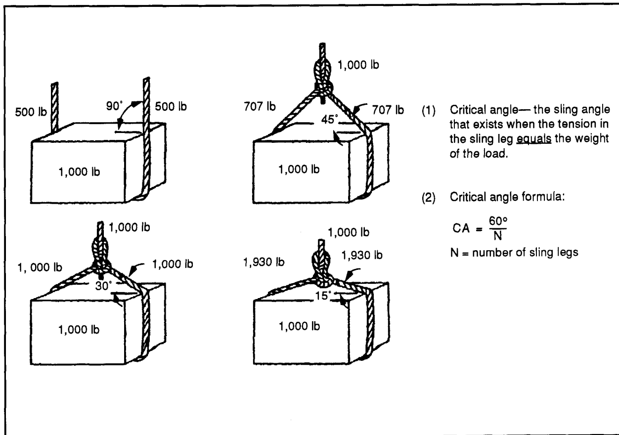
Figure 3-9. Sling angles
