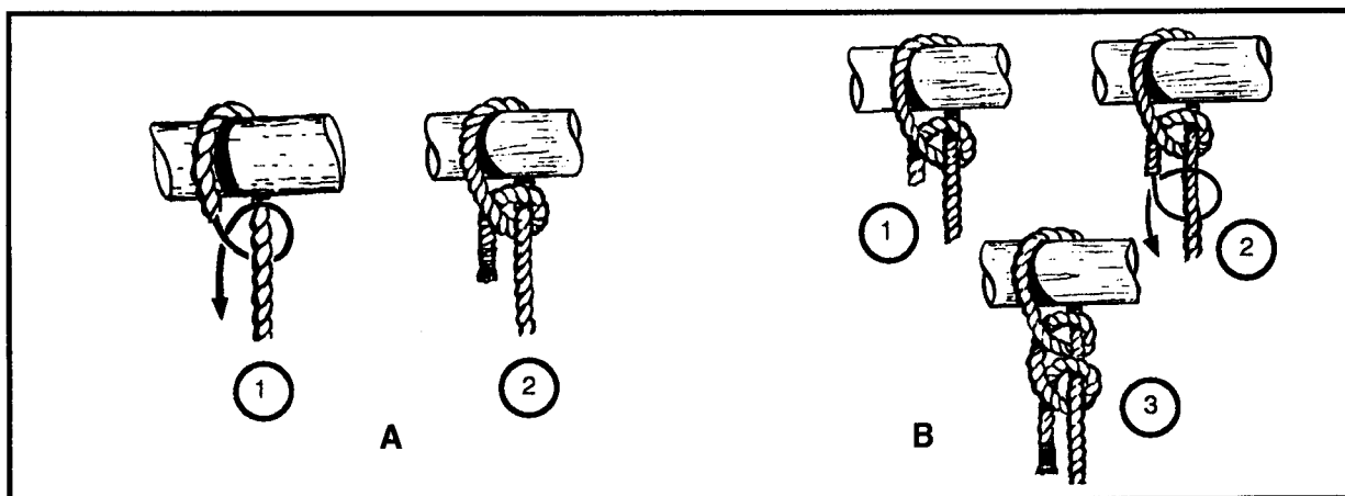
Figure 2-22. Half hitches
