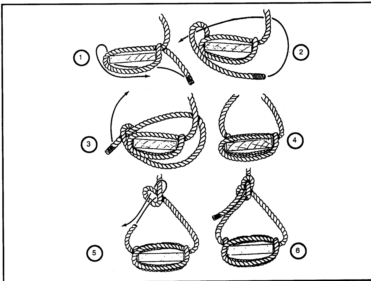
Figure 2-30. Scaffold hitch
