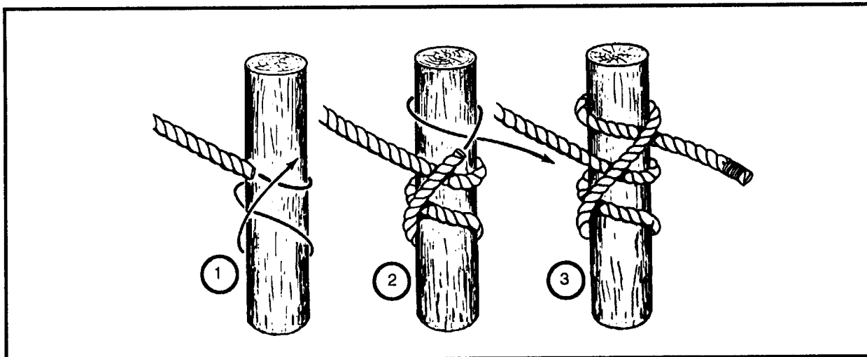
Figure 2-29. Mooring hitch
